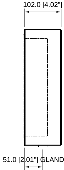
RIGHT SIDE VIEW PANEL PC SHOWN PHANTOM
