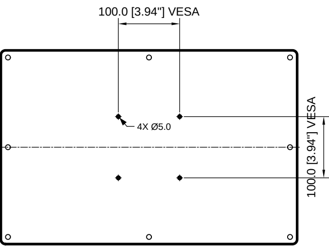
REAR VIEW REMOVABLE COVER, 8 SCREWS
