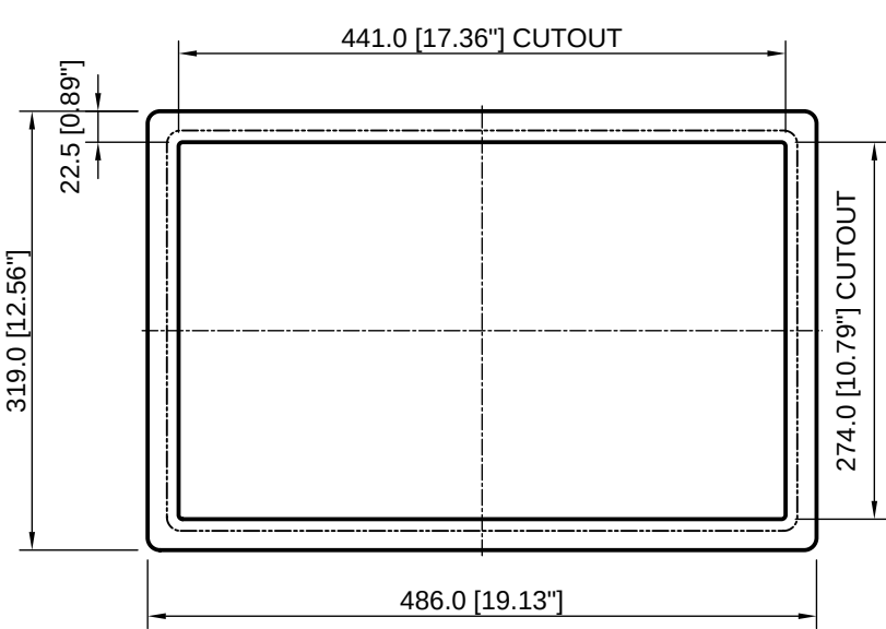
FRONT VIEW DISPLAY SHOWN PHANTOM
